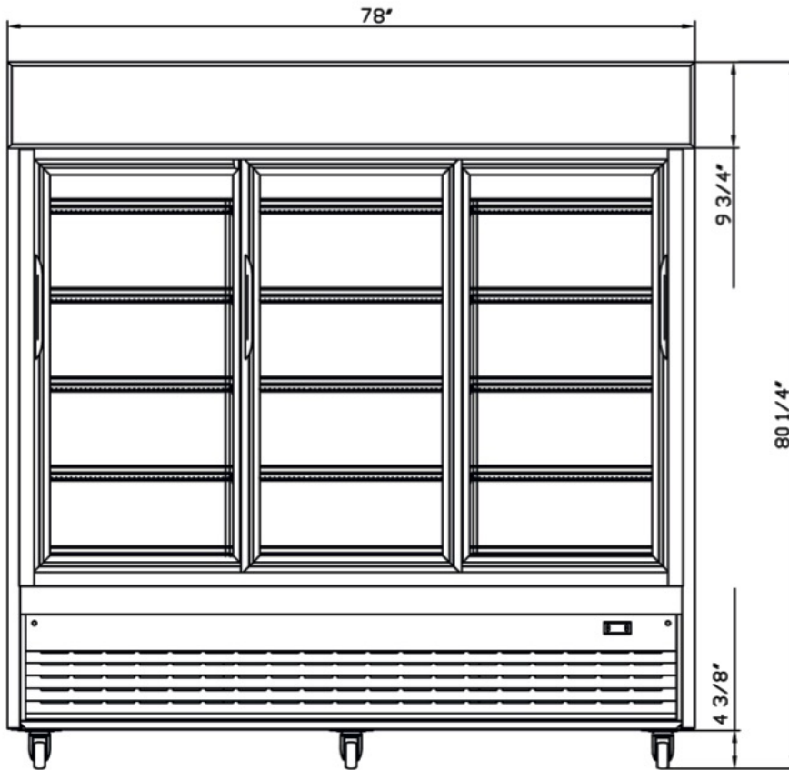
Front View
