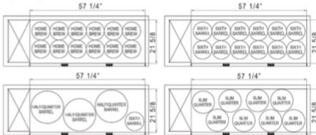
Keg configuration
