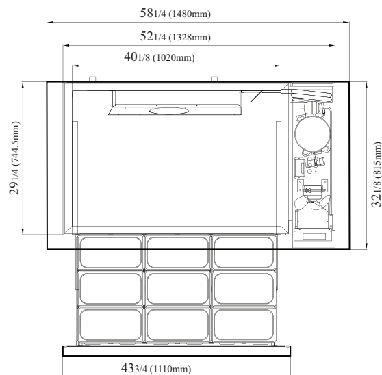
EXTENDED TOP VIEW
