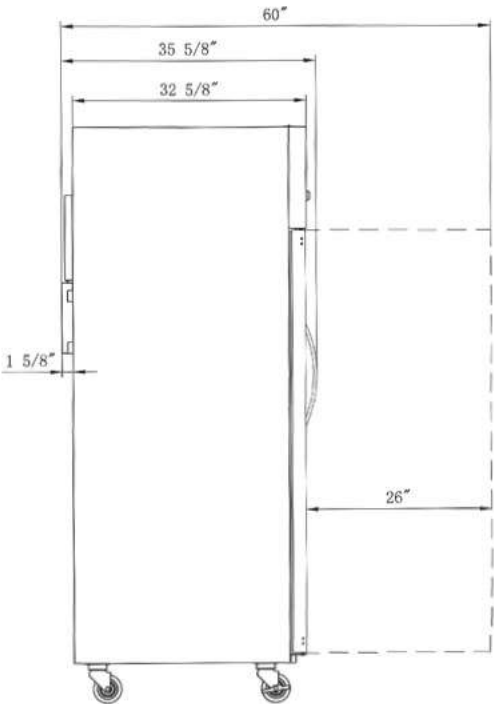
Side View
