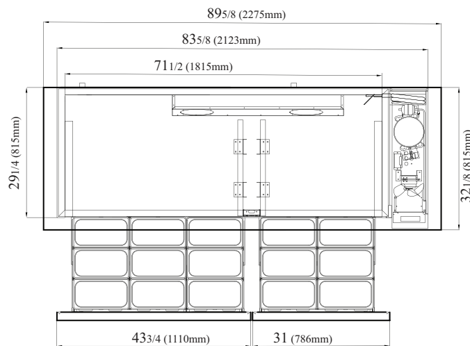
EXTENDED TOP PLAN VIEW
