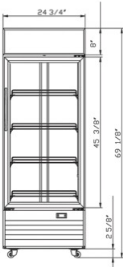
Front View
